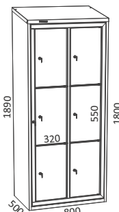
Ref. 160 6 TI
