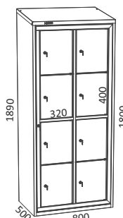
Ref. 160 8 TI
