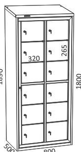
Ref. 160 12 2 TI
