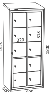
Ref. 160 10 2 TI
