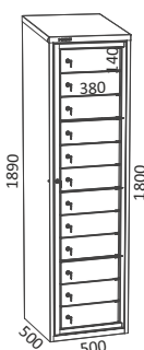
Ref. 160 8 TI
