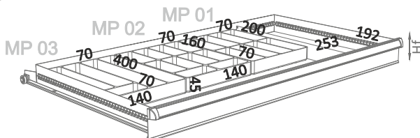
Ref. 143 MP 01-02-03 Hf 075-100
