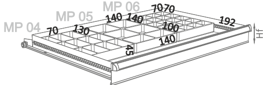
Ref. 119 MP 04-05-06 Hf 075-100
