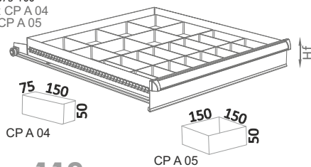
Ref. 115 075 C4 Hf 075-100 4x CPA 10 4x CPA 11 8x CPA 12
