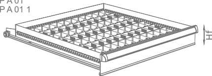
Ref. 115 075 C3 Hf 075-100 16x CPA 04 8x CPA 05
