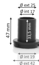
Ref. CAPTO 8
