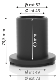
Ref. HSK 100
