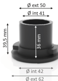
Ref. VDI 40
