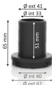
Ref. HSK 80
