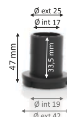
Ref. CAPTO 8
