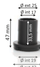
Ref. CAPTO 8
