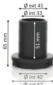
Ref. HSK 80
